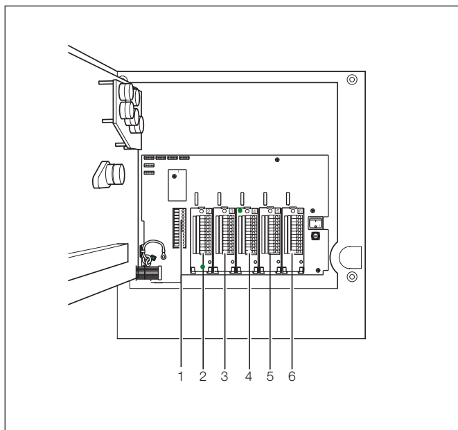
Module Positions
