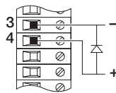
c - Current (non 2-wire Transmitters)
